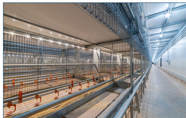
Rope lights can provide uniform lighting to brooding sections in aviary systems.
